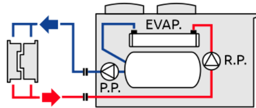
S: with tank, recirculating and process pumps
