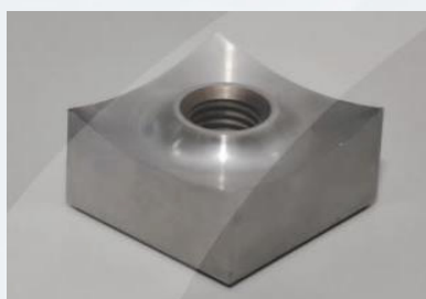
The shredders use concave ground square knives, producing high quality output. The cutters can be turned after a side is worn out.
