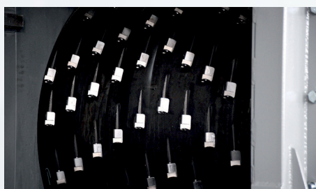
The ZRS uses very large diameter flat E-style rotors. Knives are fixed in special knife holders fitted in machined pockets.
